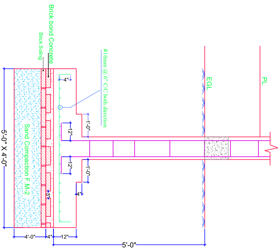
Section of Footing-2
