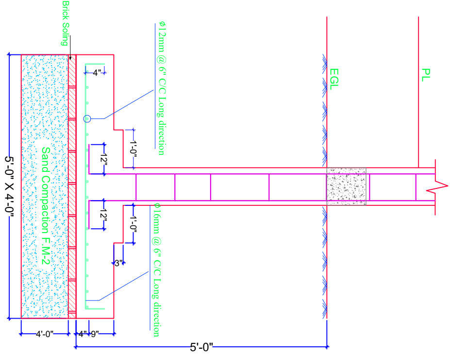
Section of Footing-1
